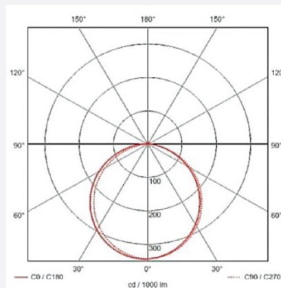
Photometric curve
