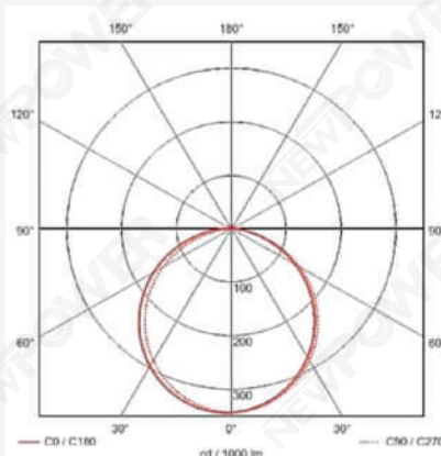
Photometric curve
