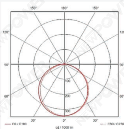
Photometric curve
