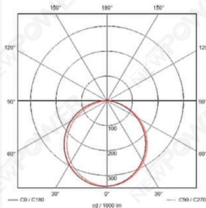
Photometric curve
