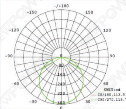
Photometric curve
