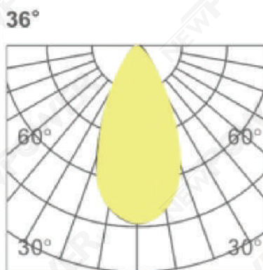
Photometric curve
