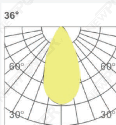
Photometric curve
