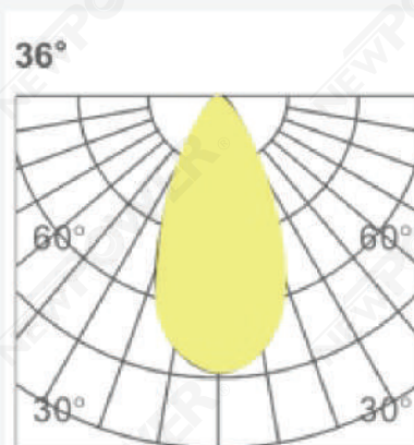
Photometric curve
