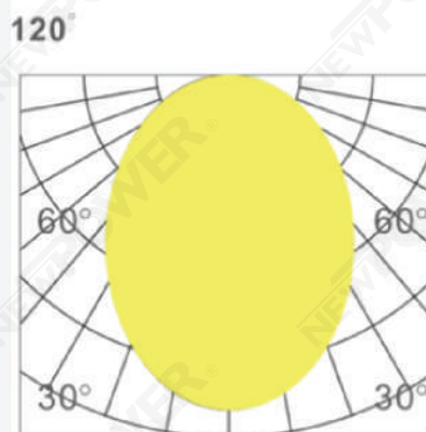
Photometric curve
