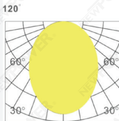
Photometric curve
