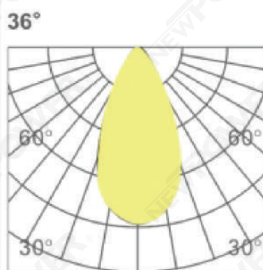
Photometric curve
