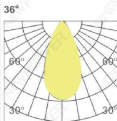
Photometric curve
