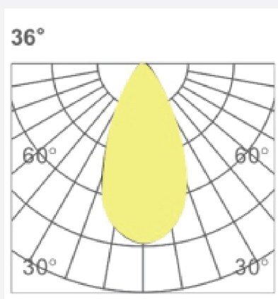
Photometric curve
